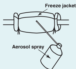
Figure 3 Disposable freezer kit
