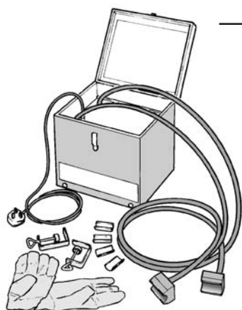
Figure 1 Typical pipe-freezing machine.
