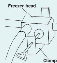
Figure 4 Freezer head clamped to pipe
